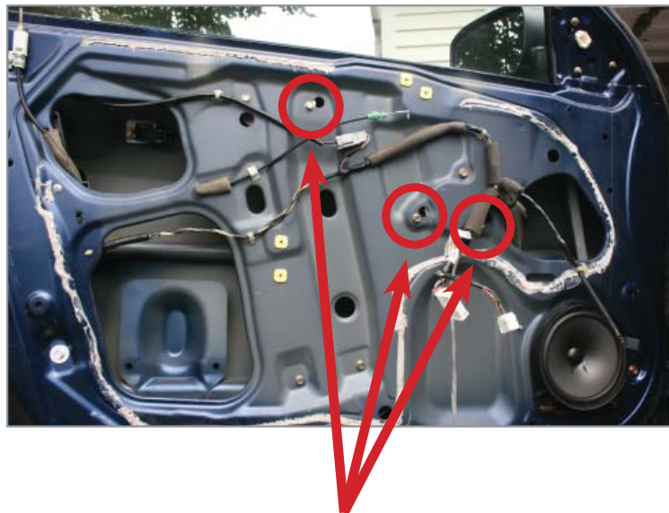
Support Regulator by hanging it on the three started bolts
