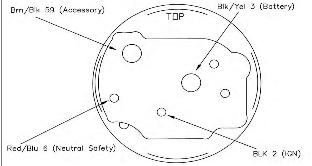
Figure 7-42 1968 - 1970 Ford Truck Ignition Switch
