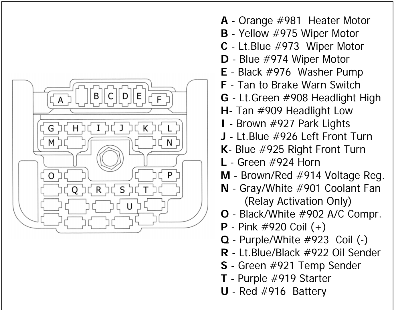
Illustration 3 Engine Harness Firewall Connector Style #2
