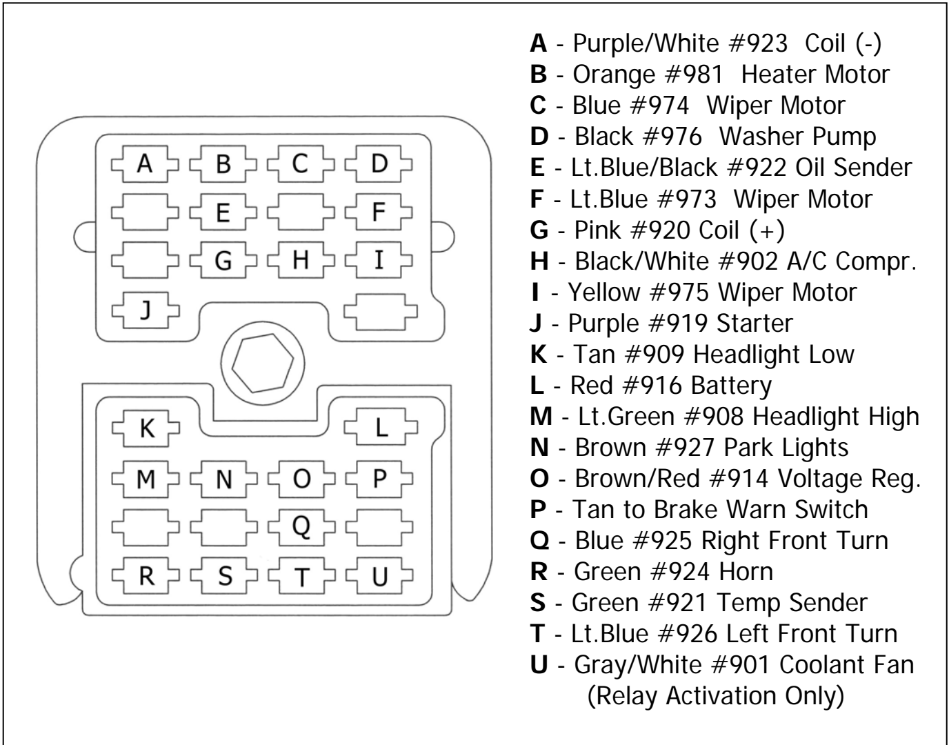
Illustration 2 Engine Harness Firewall Connector Style #1
