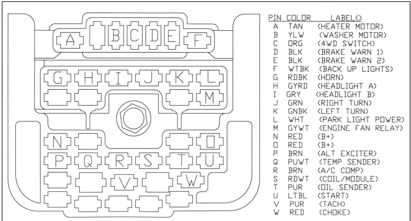
Illustration 3 Engine Harness Firewall Connector Style #2
